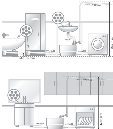
Fig. 31 Examples of installation
