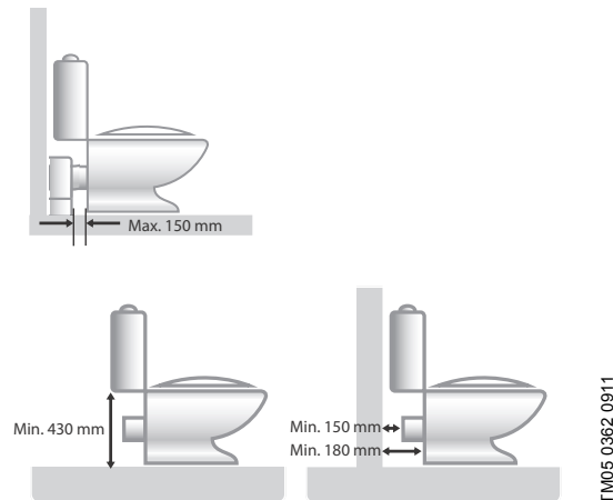
Fig. 15 Measurements to be observed
