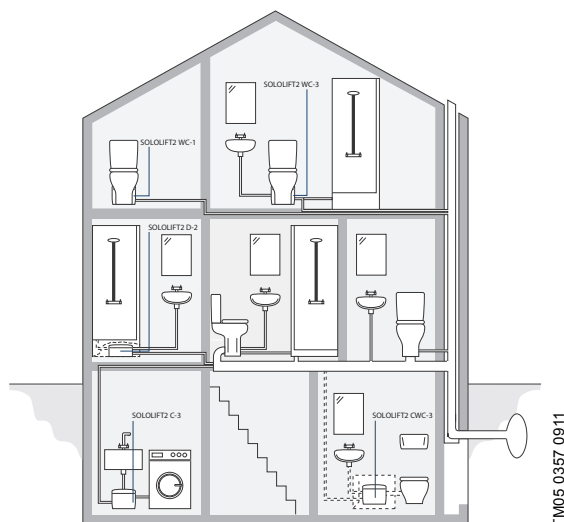
Fig. 1 Examples of application
