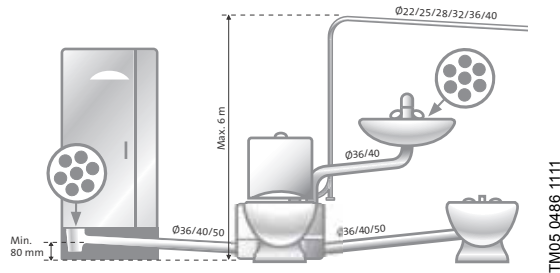
Fig. 14 Example of installation
