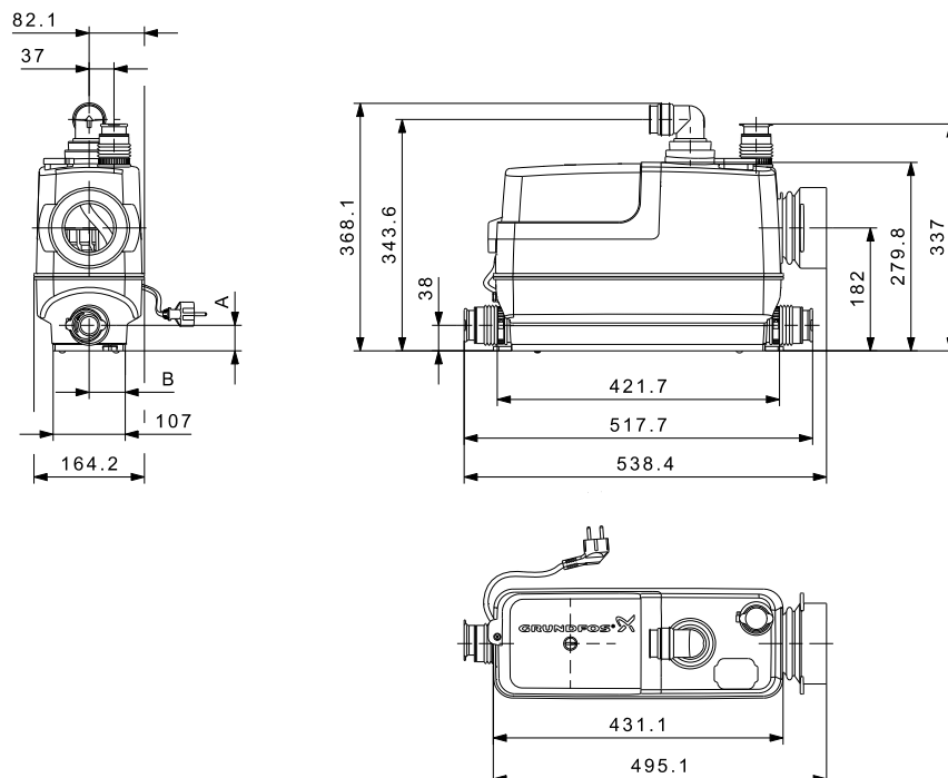
Fig. 27 Dimensional drawings, Sololift2 CWC-3
