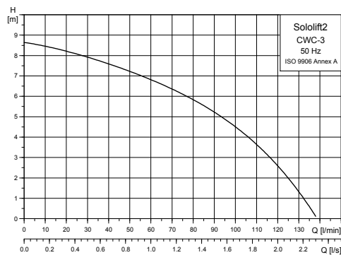
Fig. 26 Performance curves, Sololift2 CWC-3
