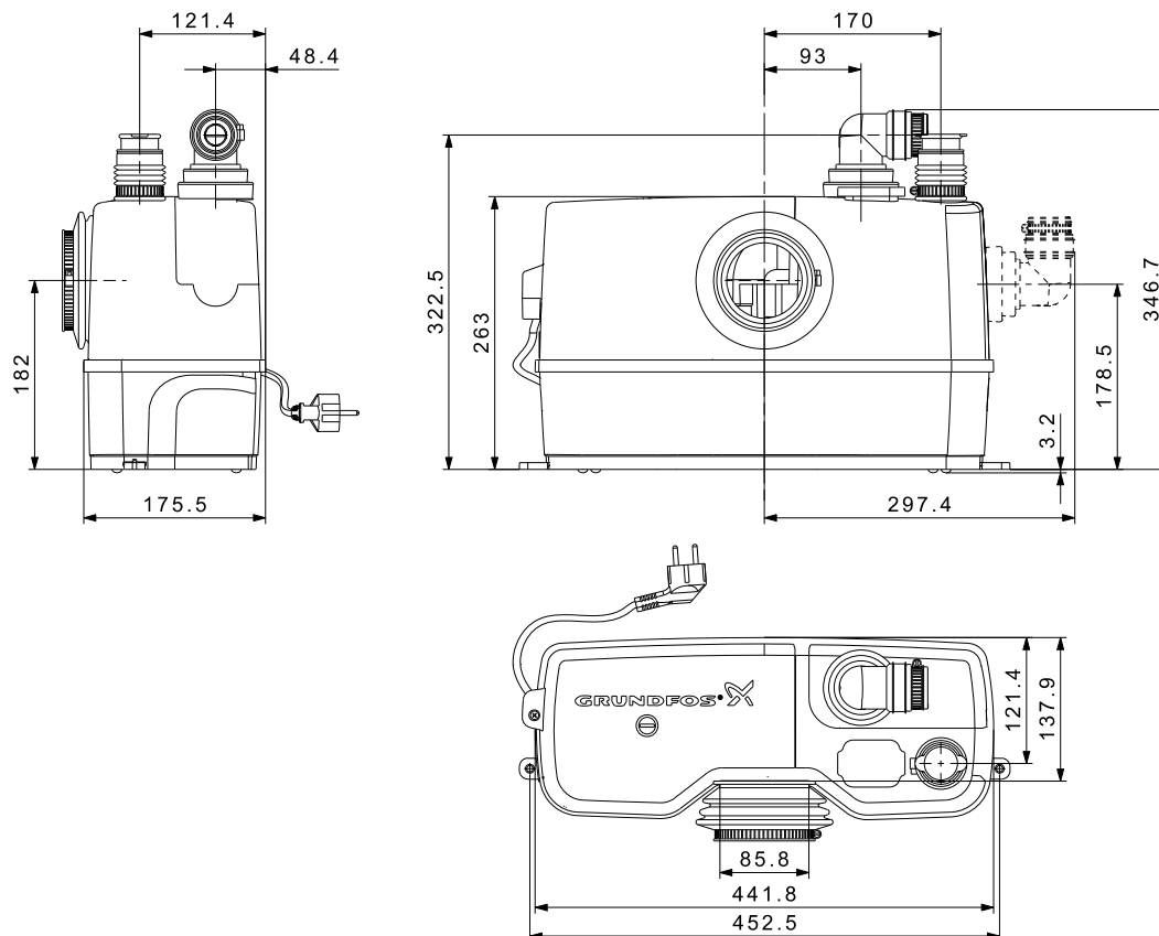
Fig. 10 Dimensional drawings, Sololift2 WC-1
