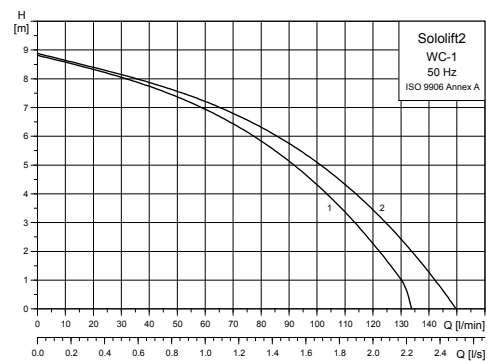
Fig. 9 Performance curves, Sololift2 WC-1
