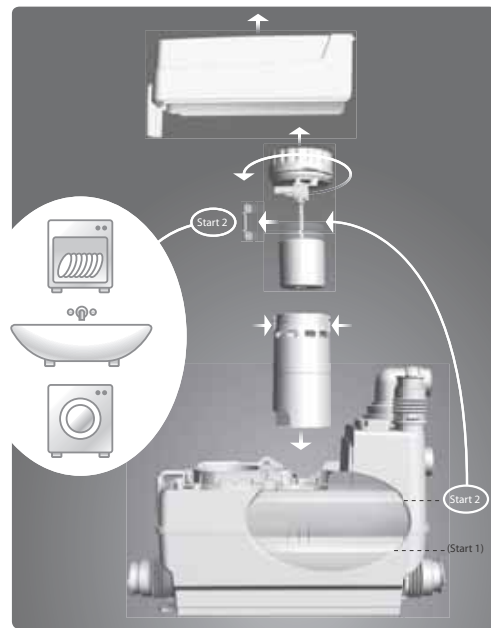
Fig. 33 Adjustment of the float switch
