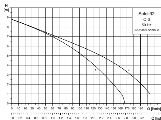
Fig. 36 Performance curves, Sololift2 C-3
