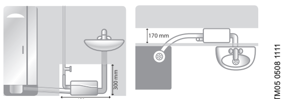
Fig. 42 Measurements to be observed
