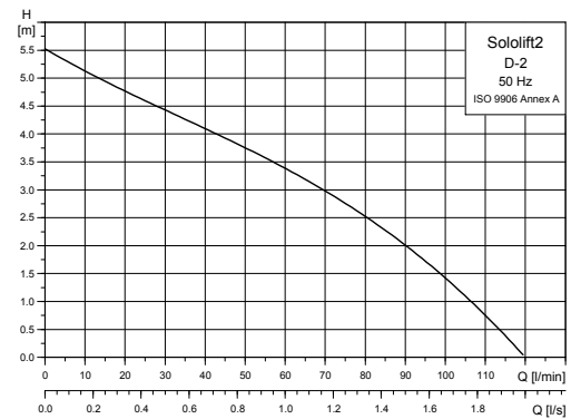
Fig. 43 Performance curves, Sololift2 D-2
