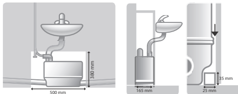
Fig. 32 Measurements to be observed
