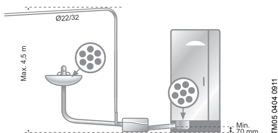
Fig. 41 Example of installation
