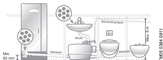
Fig. 23 Example of installation
