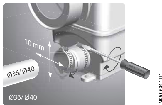
Fig. 25 Height and side alignment possible when using Ø36/40 inlet pipes
