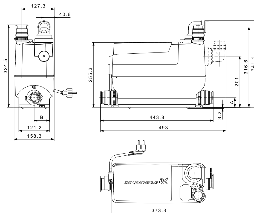
Fig. 37 Dimensional drawings, Sololift2 C-3
