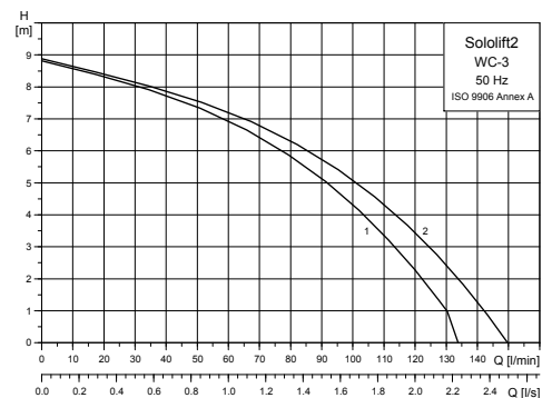
Fig. 18 Performance curves, Sololift2 WC-3
