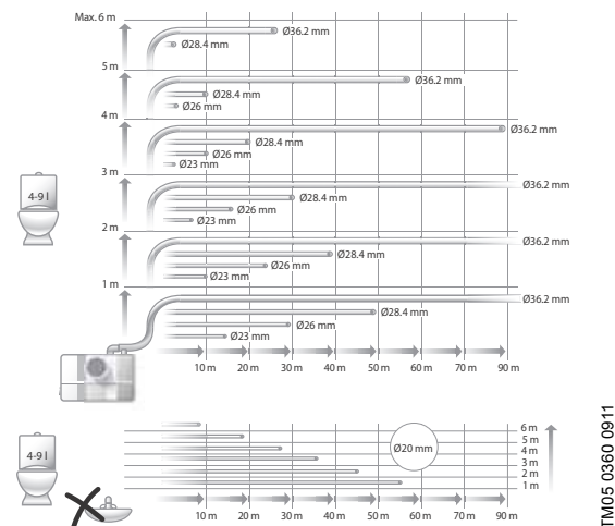
Fig. 5 Maximum lengths of vertical and horizontal discharge pipes
