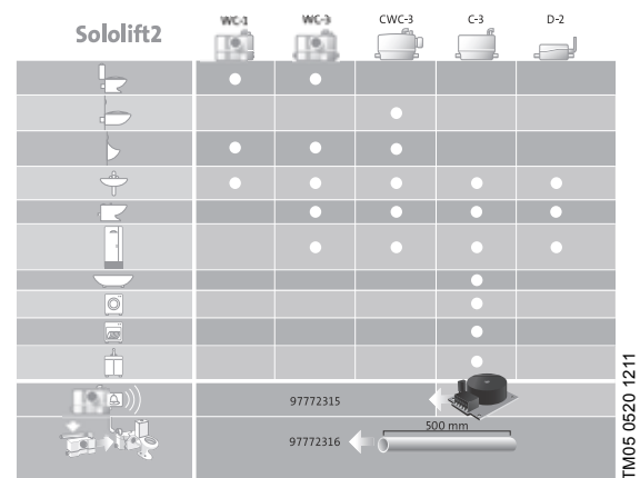
Fig. 2 Overview of Sololift2 lifting stations
